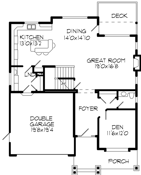
MAIN FLOOR PLAN 1190 SQ.FT.
